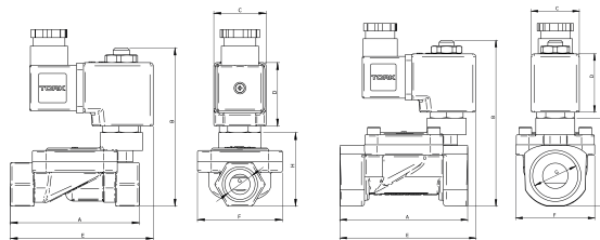
Dimensions (mm)
